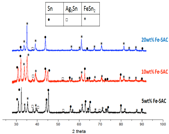
Figure 1. XRD spectra of melted Fe-SAC 305 samples.
